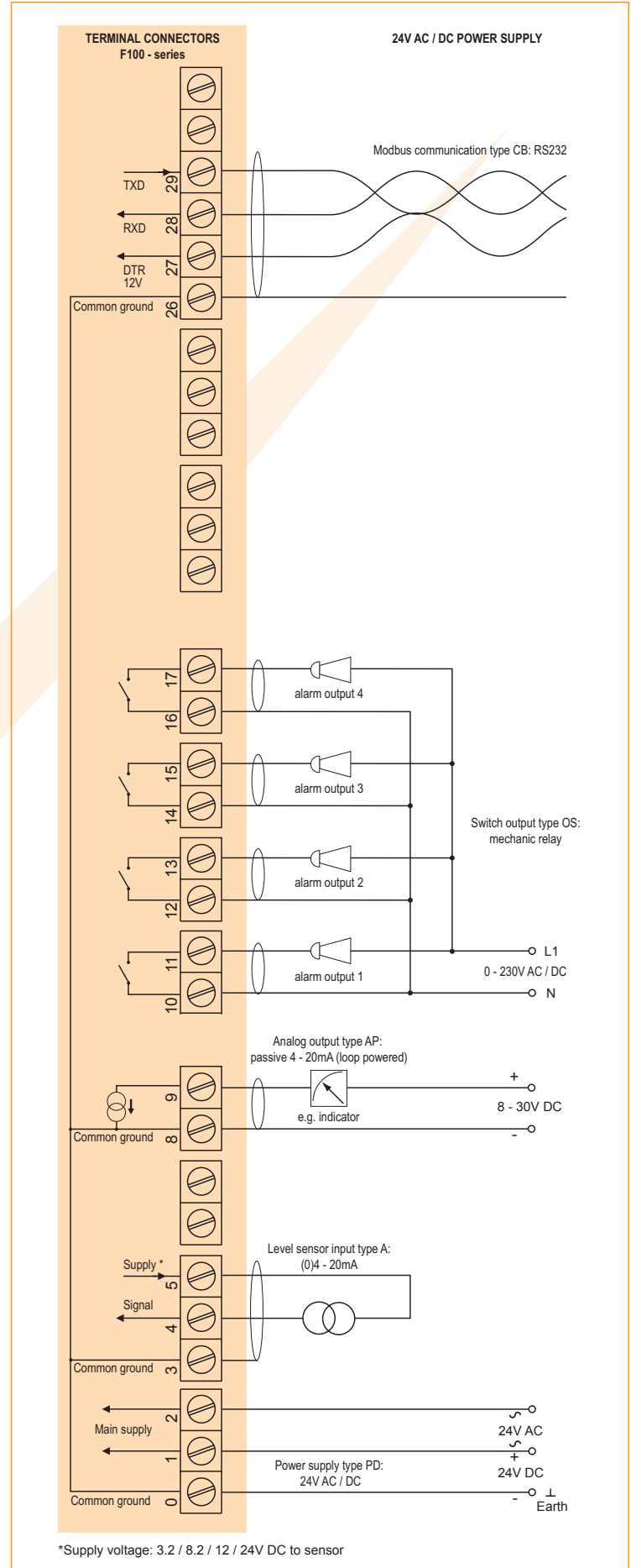
Typical wiring diagram F173-A-AP-CB-OS-PD
