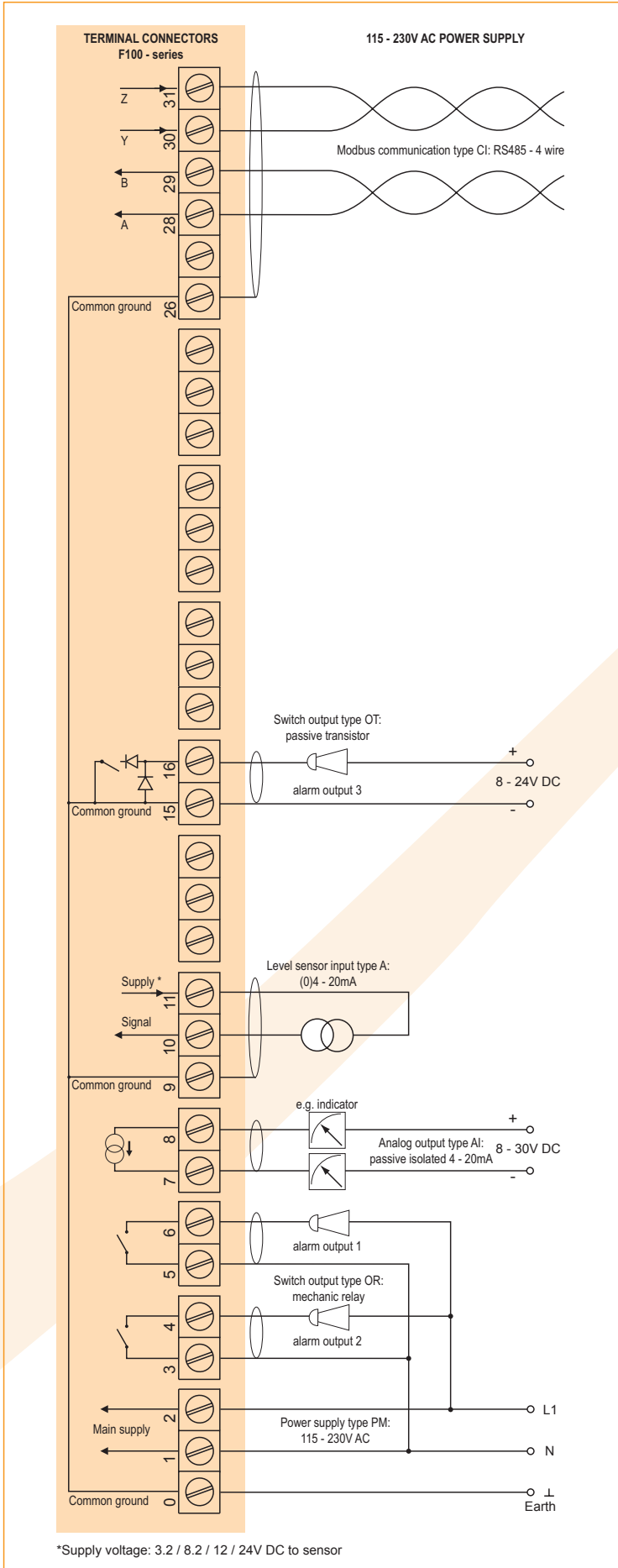
Typical wiring diagram F173-A-AI-CI-OR-PM
